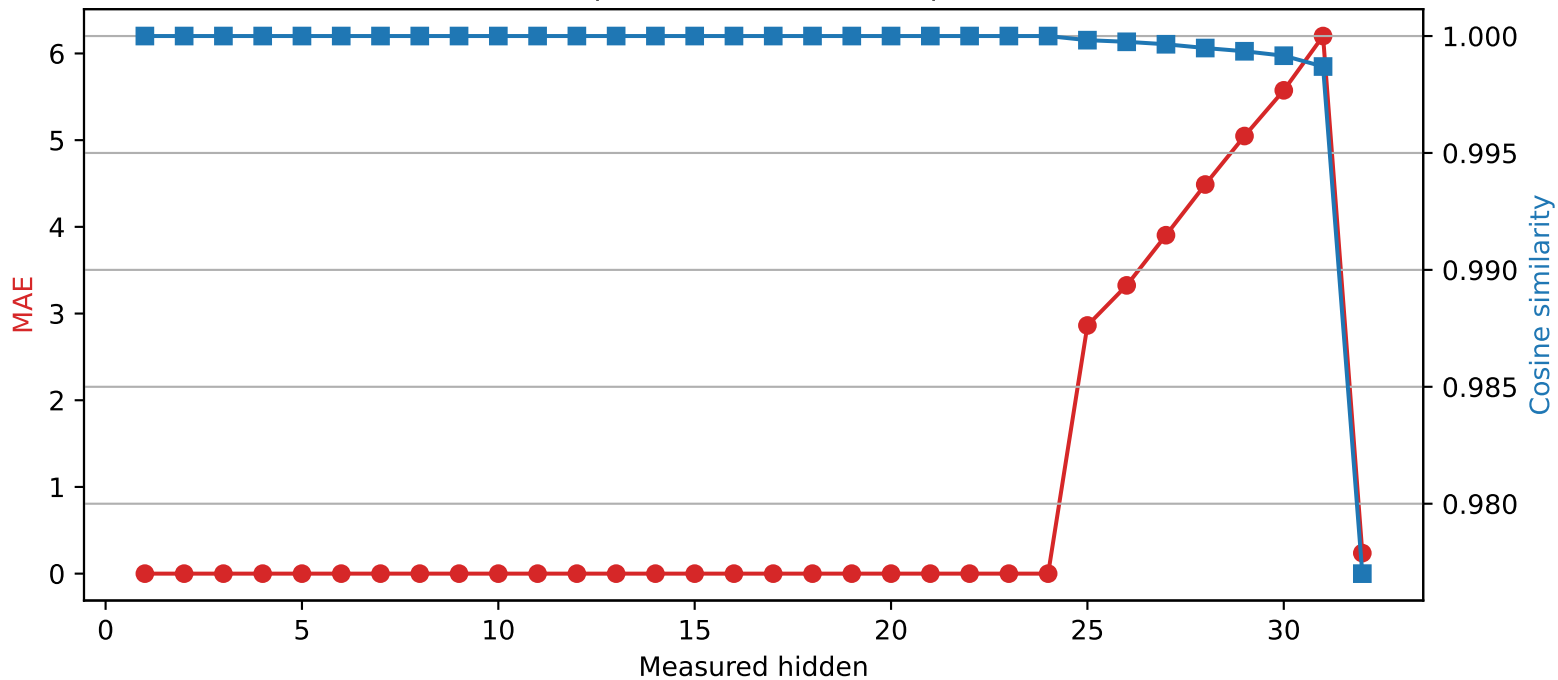
SmolLM2-360M | Quantized layer 24 | float64 → int2
