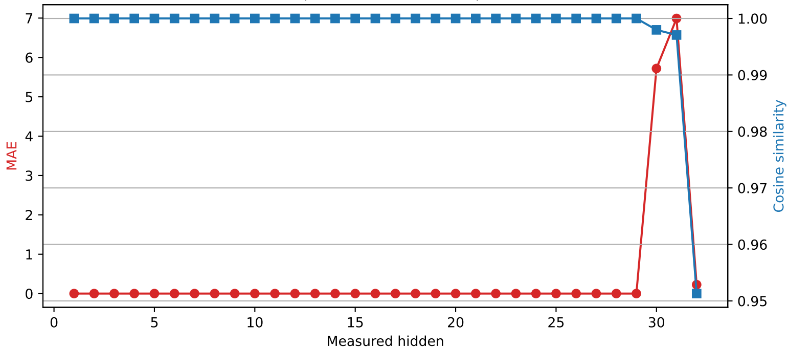
SmolLM2-360M | Quantized layer 29 | float64 → int2
