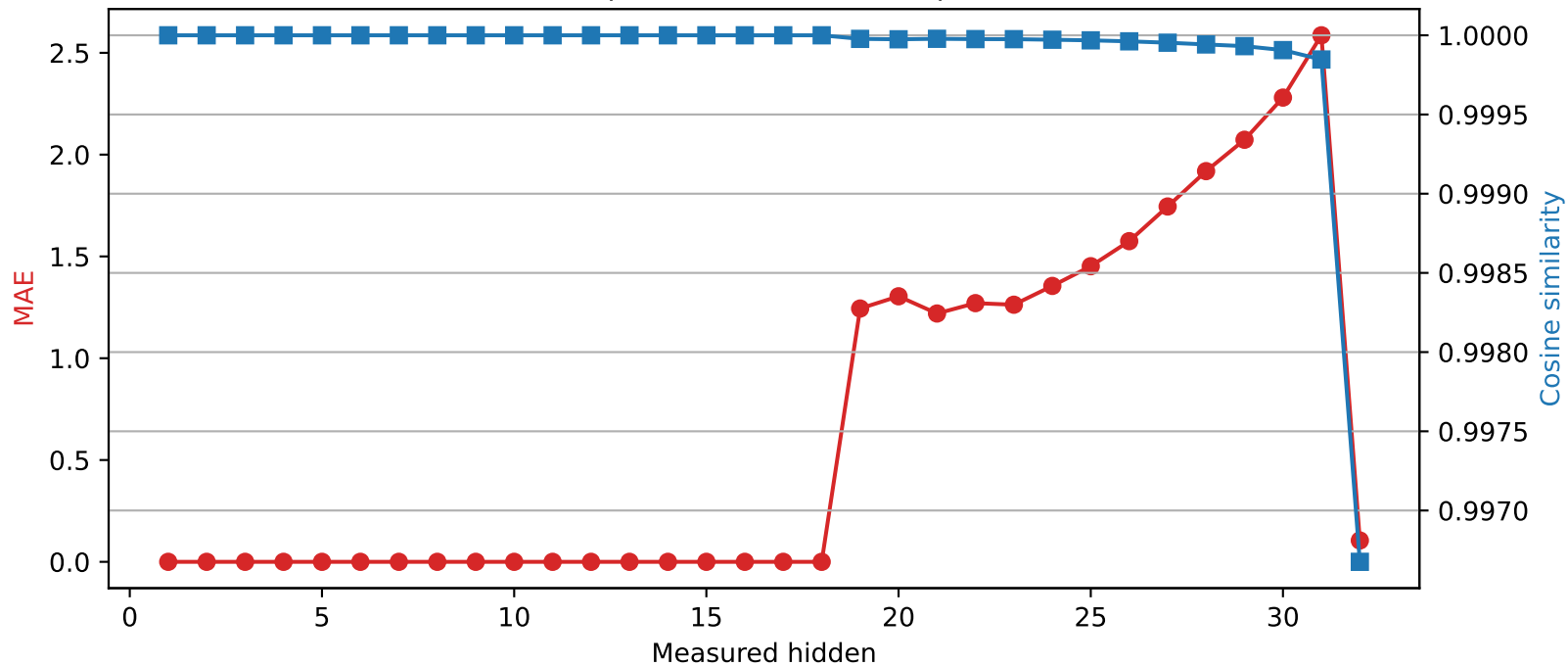
SmolLM2-360M | Quantized layer 18 | float64 → int2
