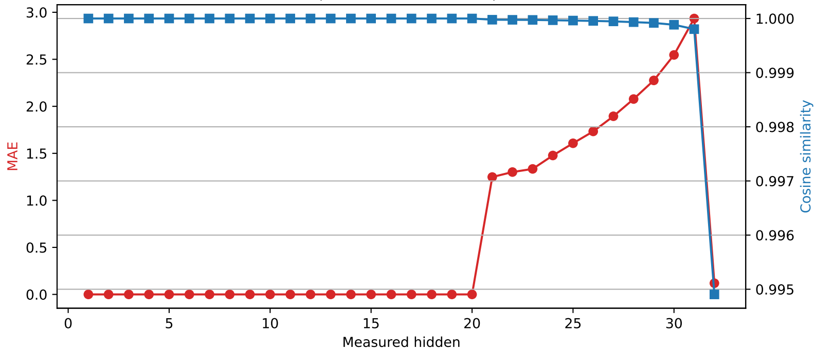
SmolLM2-360M | Quantized layer 20 | float64 → int2
