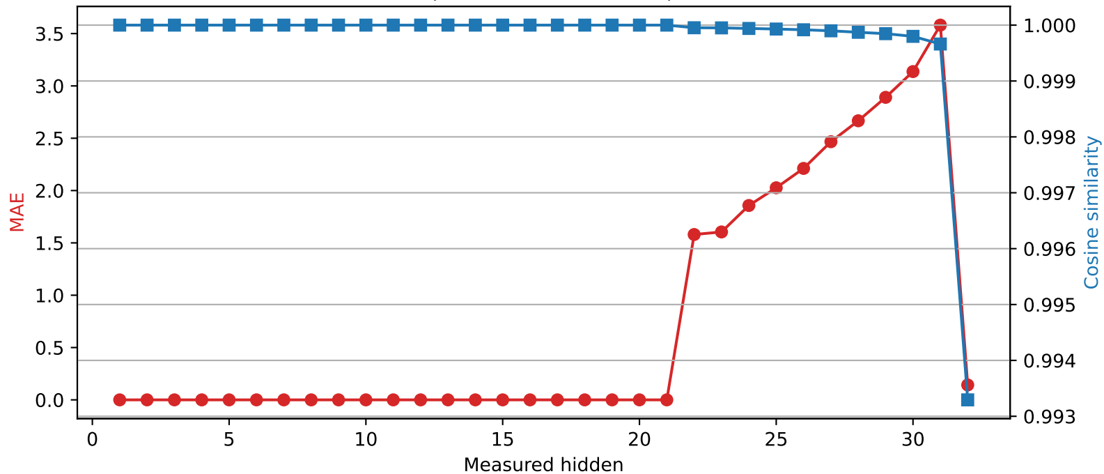
SmolLM2-360M | Quantized layer 21 | float64 → int2
