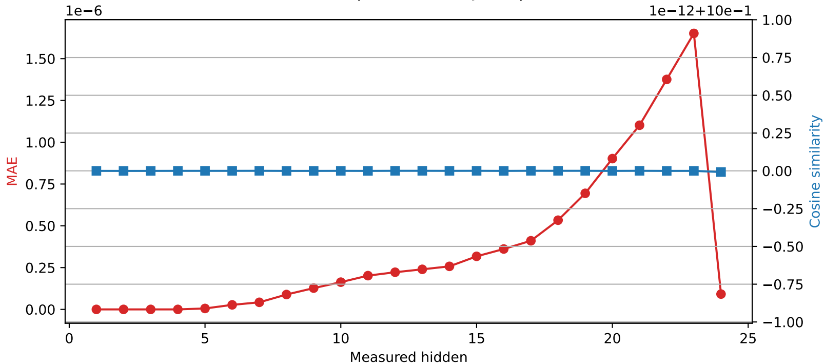
SmolLM2-1.7B-Instruct | Quantized layer 4 | float64 → int32
