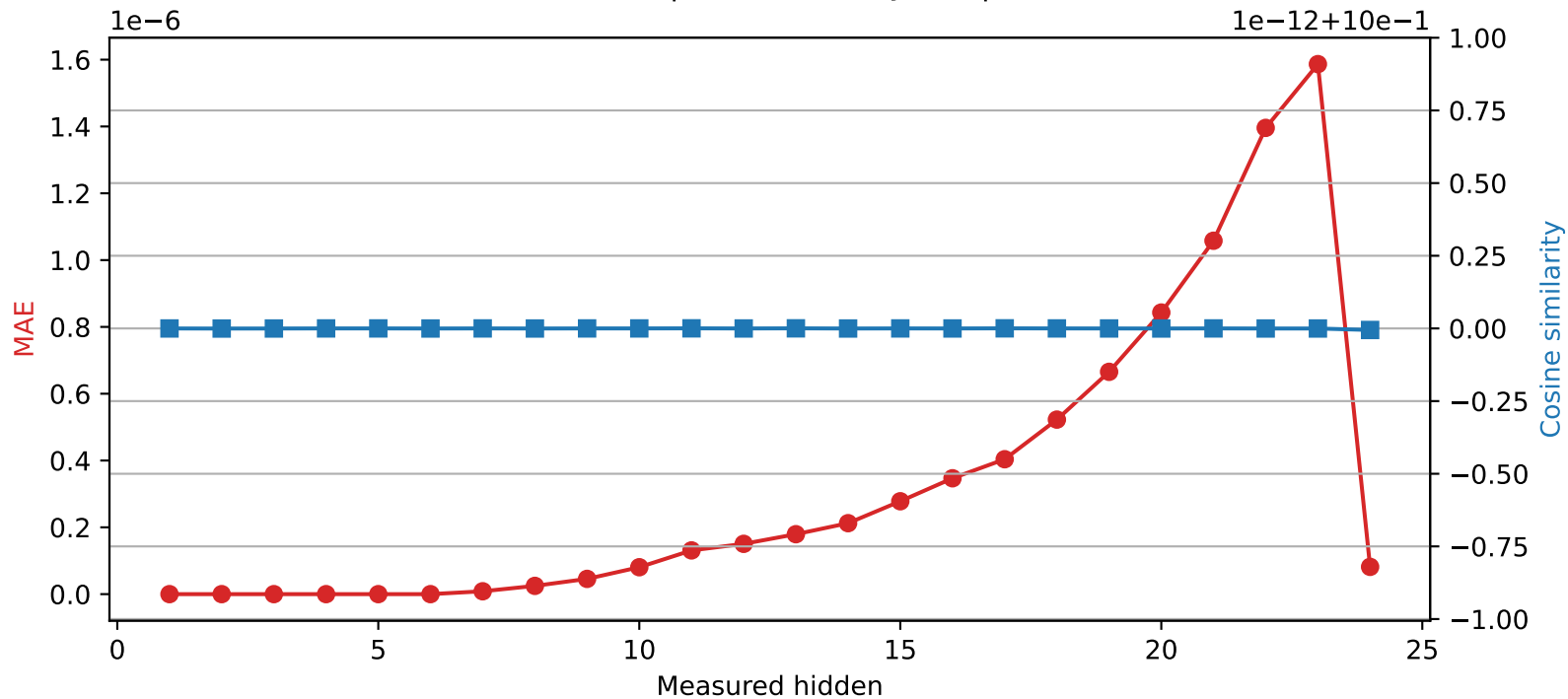
SmolLM2-1.7B-Instruct | Quantized layer 6 | float64 → int32
