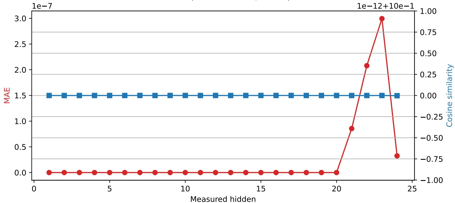
SmolLM2-1.7B-Instruct | Quantized layer 20 | float64 → int32
