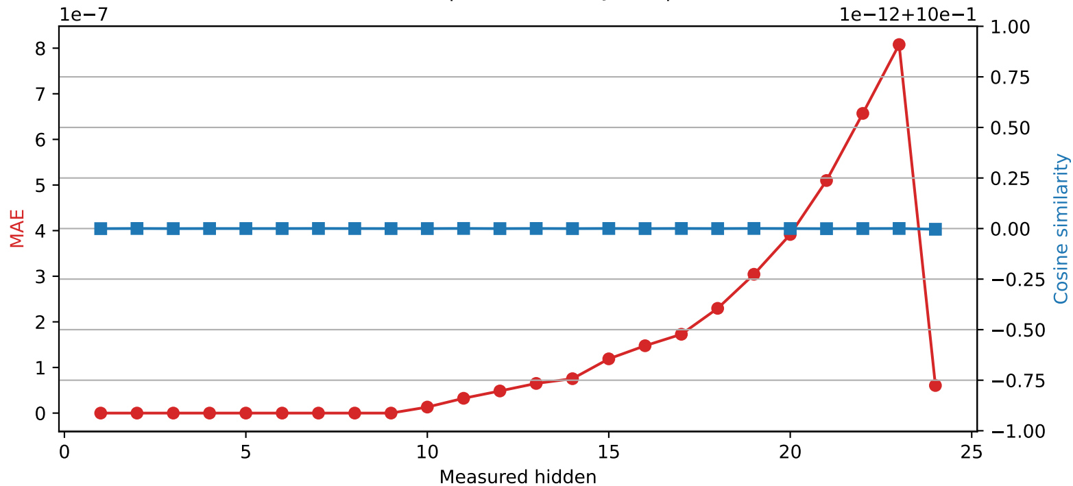
SmolLM2-1.7B-Instruct | Quantized layer 9 | float64 \rightarrow int32
