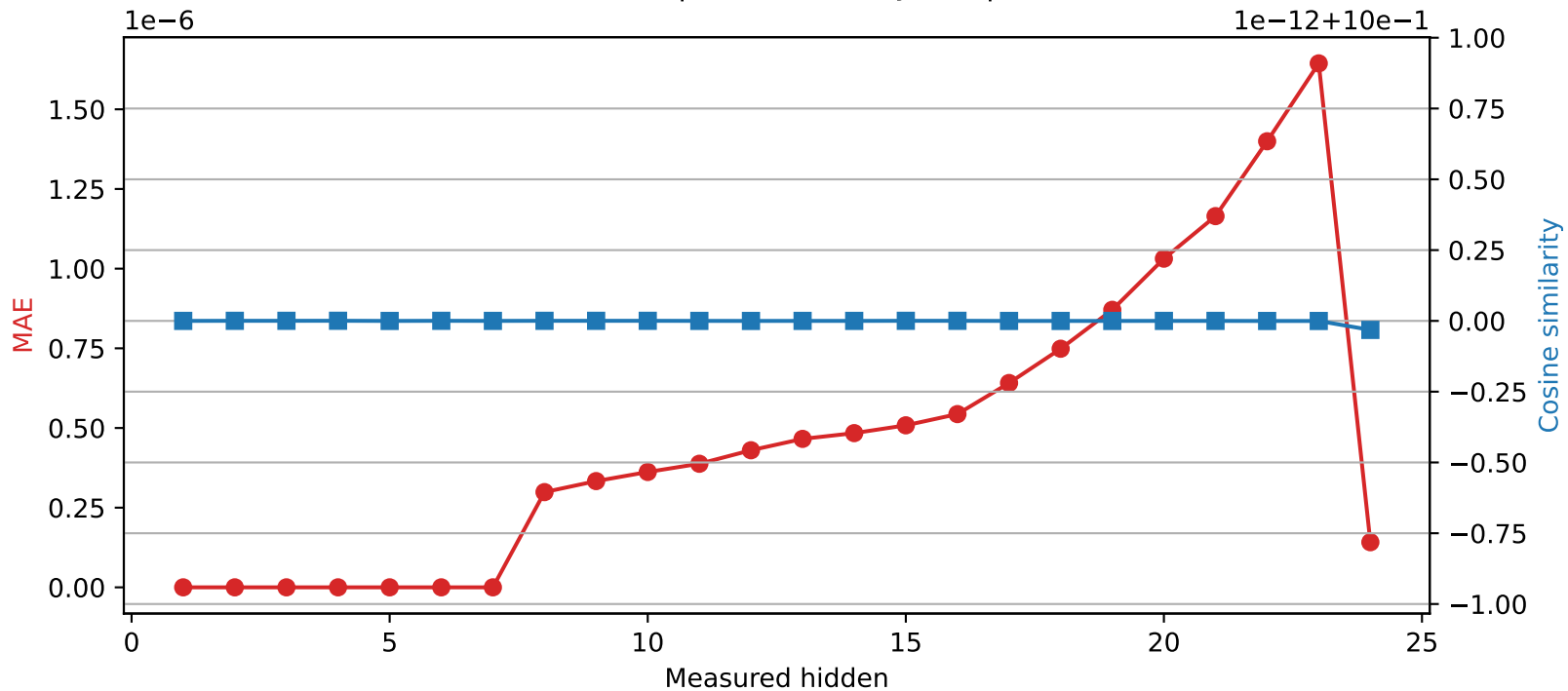
SmolLM2-1.7B-Instruct | Quantized layer 7 | float64 → int32
