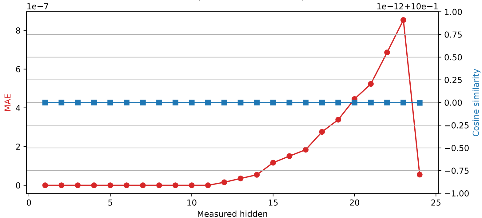
SmolLM2-1.7B-Instruct | Quantized layer 11 | float64 → int32
