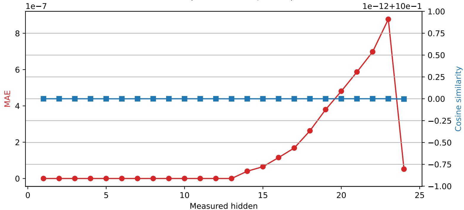
SmolLM2-1.7B-Instruct | Quantized layer 13 | float64 → int32
