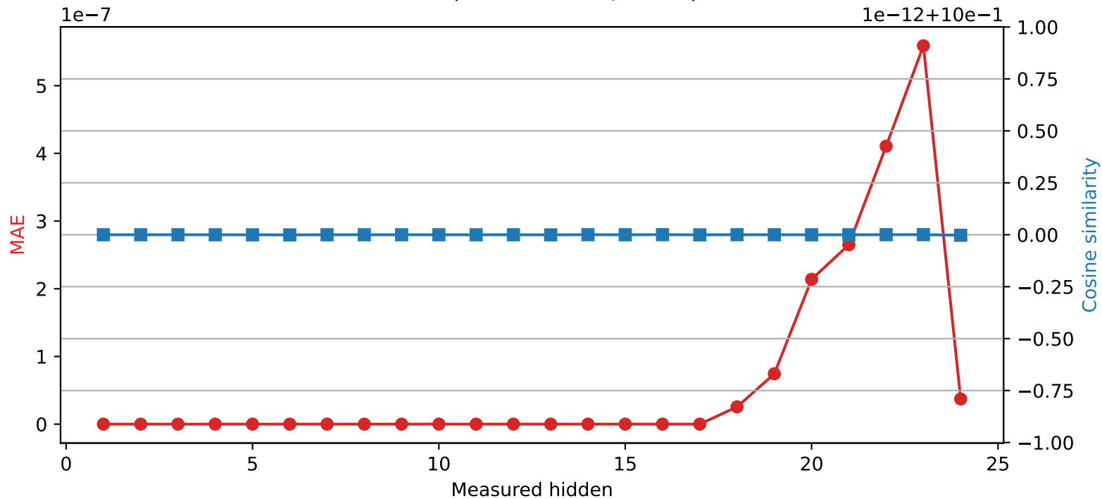
SmolLM2-1.7B-Instruct | Quantized layer 17 | float64 → int32
