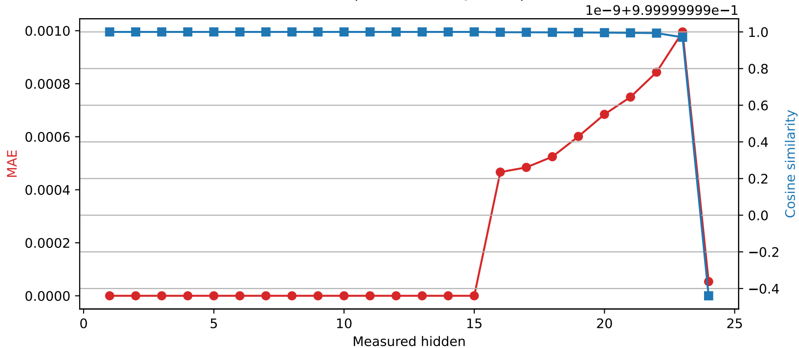
SmolLM2-1.7B-Instruct | Quantized layer 15 | float32 → int16
