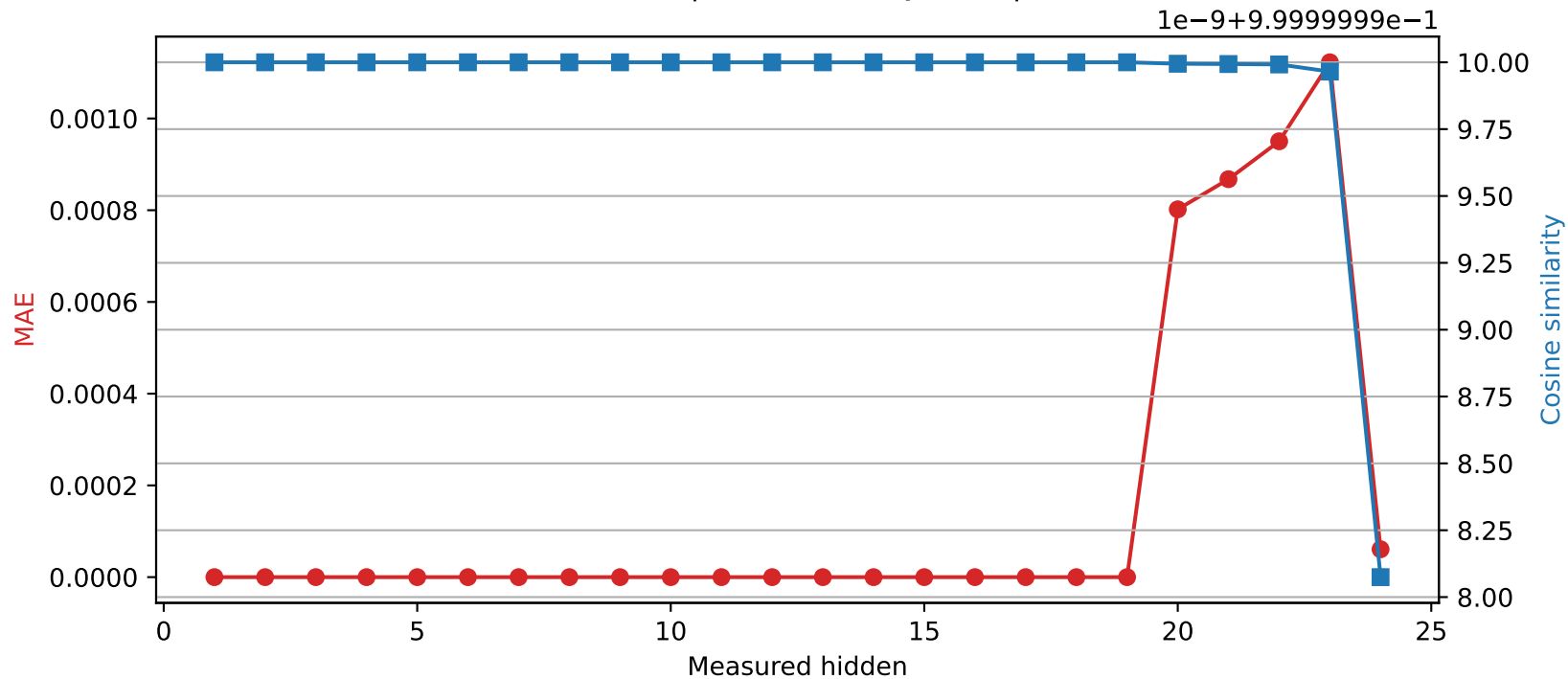
SmolLM2-1.7B-Instruct | Quantized layer 19 | float32 \rightarrow int16
