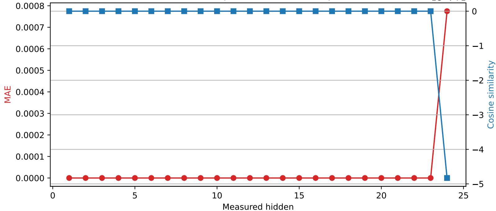
SmolLM2-1.7B-Instruct | Quantized layer 23 | float32 → int16
