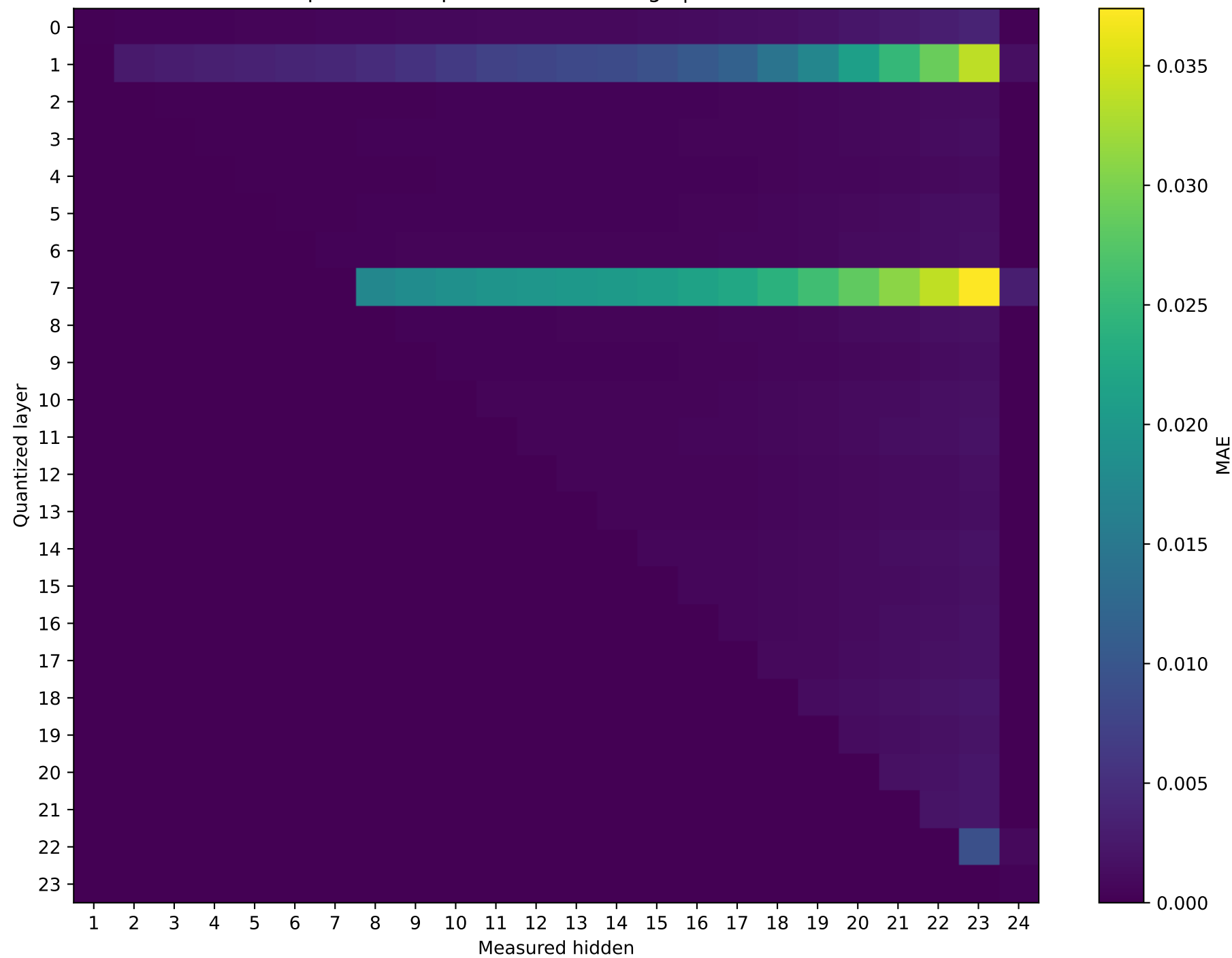
SmolLM2-1.7B-Instruct Prompt 1: MAE representation damage | float32 → int16
