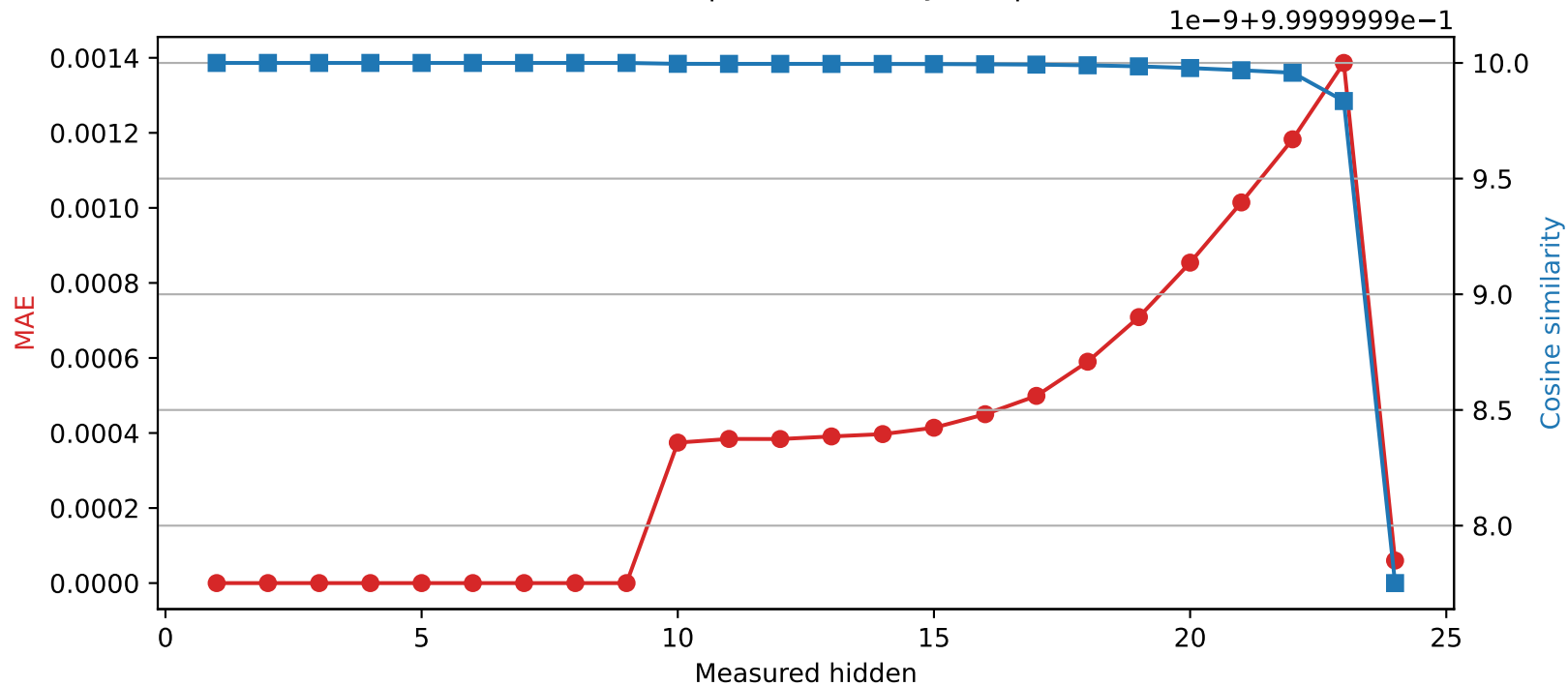
SmolLM2-1.7B-Instruct | Quantized layer 9 | float32 → int16
