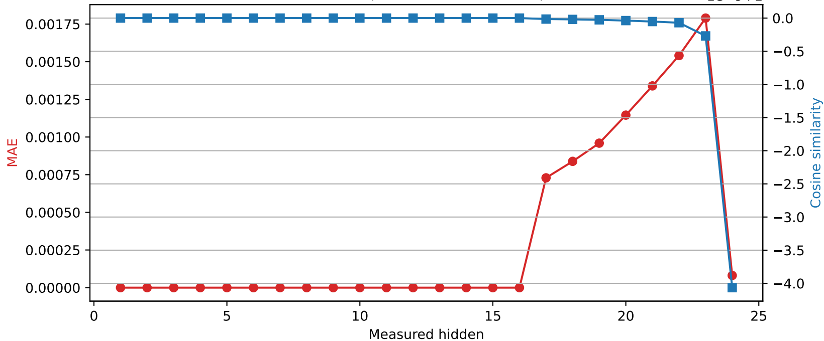
SmolLM2-1.7B-Instruct | Quantized layer 16 | float32 → int16
