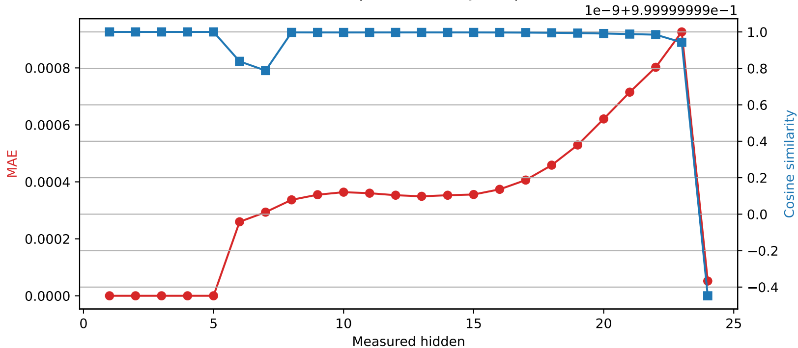
SmolLM2-1.7B-Instruct | Quantized layer 5 | float32 → int16
