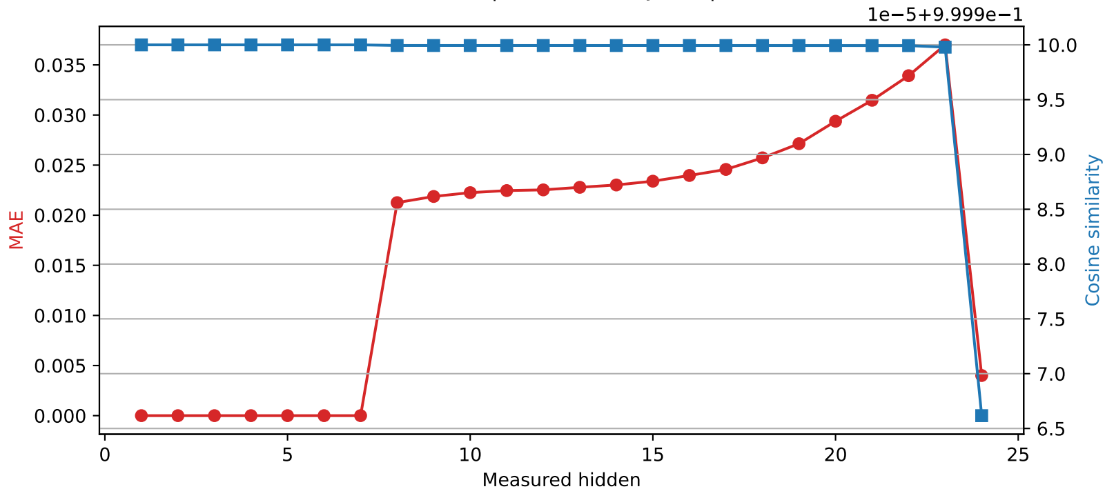
SmolLM2-1.7B-Instruct | Quantized layer 7 | float32 → int16
