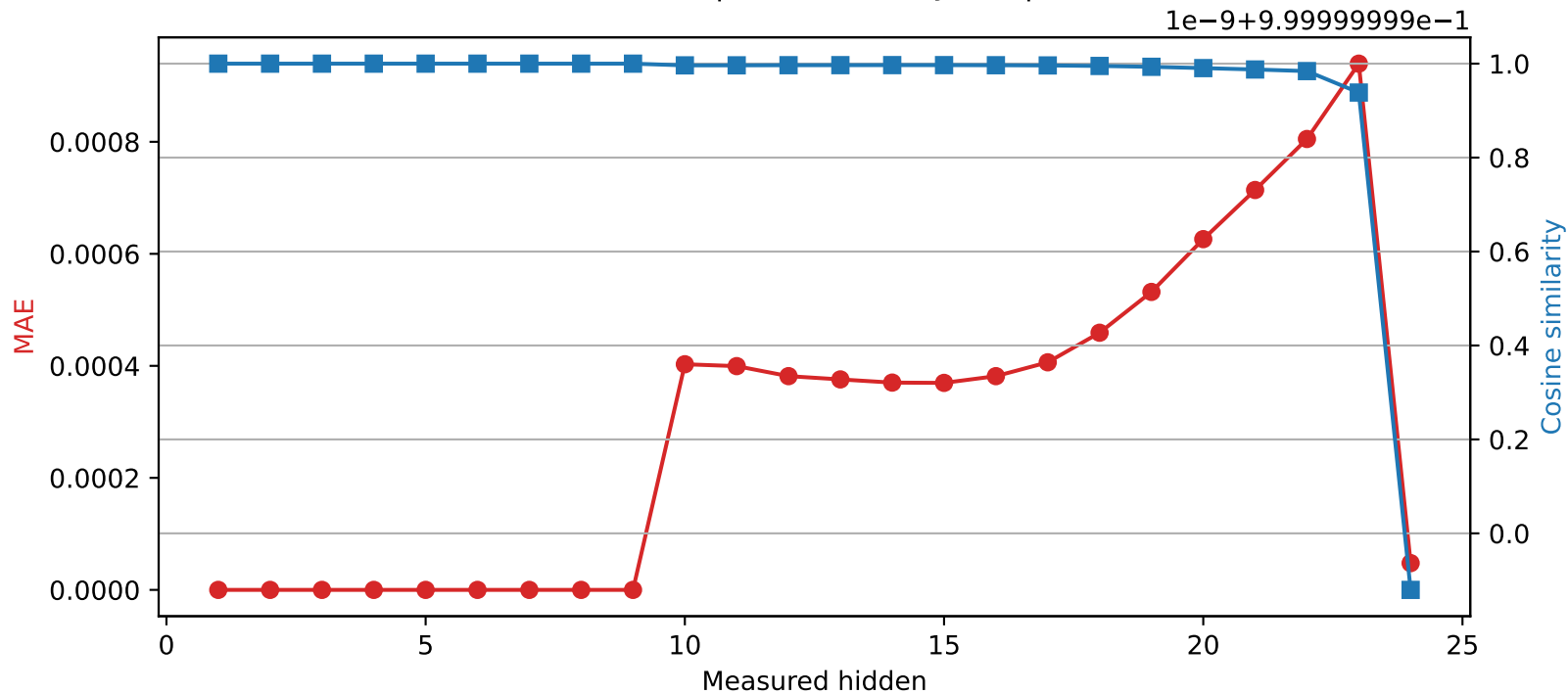
SmolLM2-1.7B-Instruct | Quantized layer 9 | float32 \rightarrow int16
