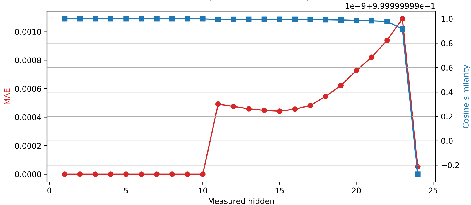
SmolLM2-1.7B-Instruct | Quantized layer 10 | float32 → int16
