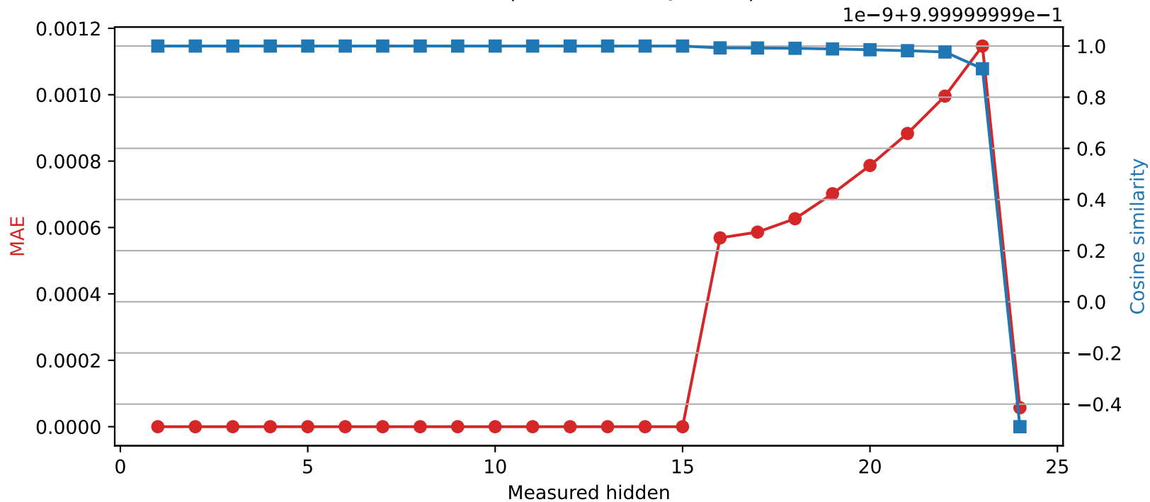
SmolLM2-1.7B-Instruct | Quantized layer 15 | float32 \rightarrow int16
