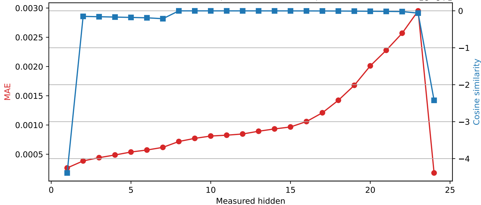
SmolLM2-1.7B-Instruct | Quantized layer 0 | float32 \rightarrow int16
