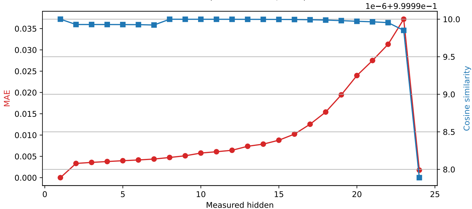
SmolLM2-1.7B-Instruct | Quantized layer 1 | float32 \rightarrow int16
