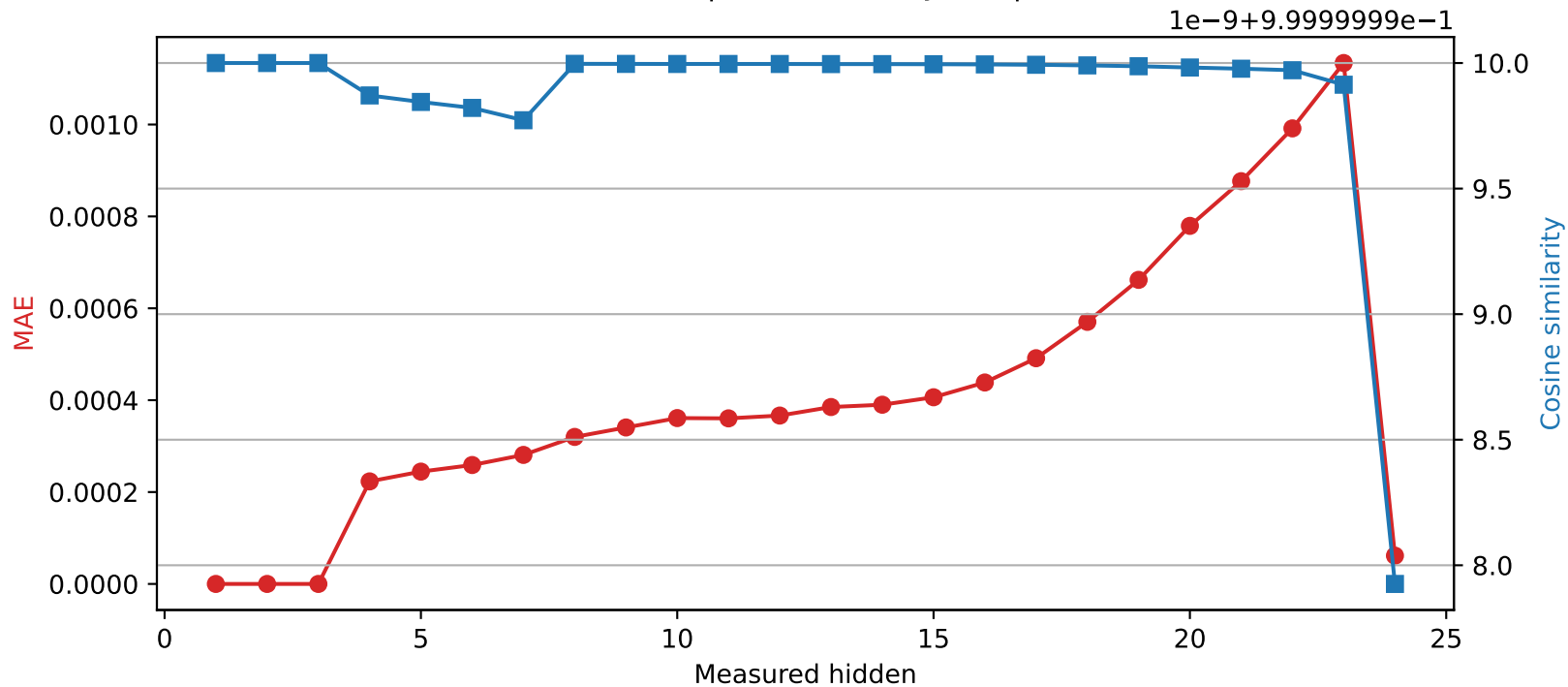
SmolLM2-1.7B-Instruct | Quantized layer 3 | float32 → int16
