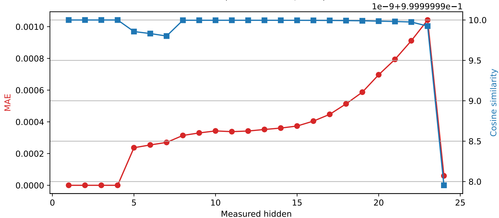
SmolLM2-1.7B-Instruct | Quantized layer 4 | float32 → int16
