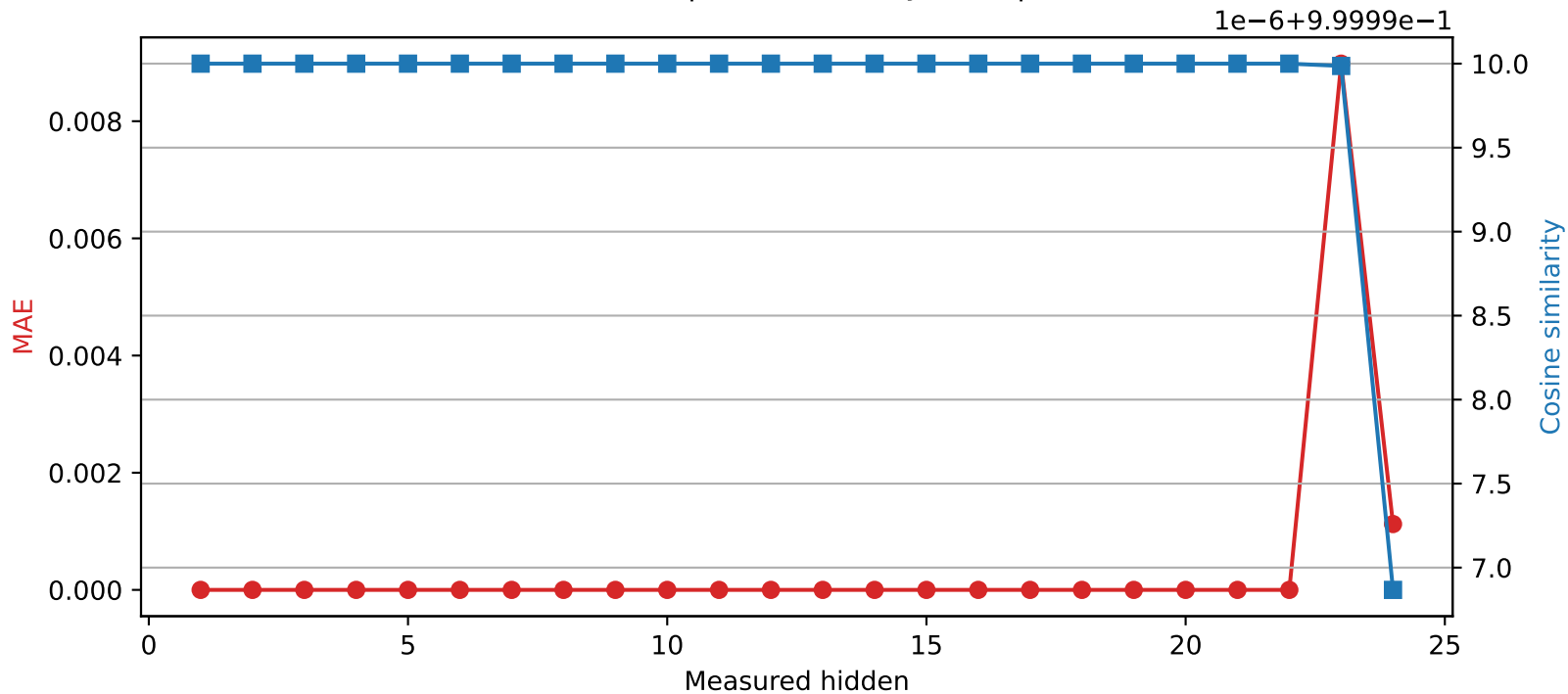
SmolLM2-1.7B-Instruct | Quantized layer 22 | float32 \rightarrow int16
