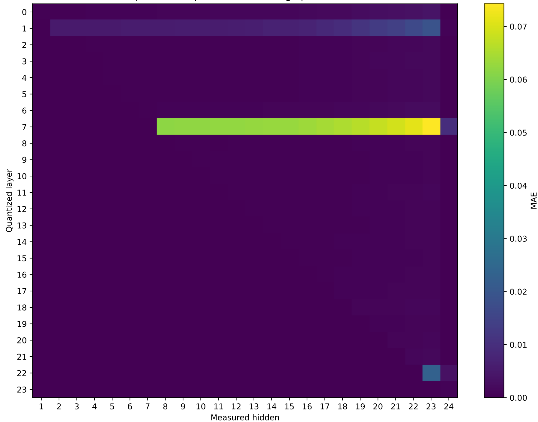
SmolLM2-1.7B-Instruct Prompt 0: MAE representation damage | float64 → int16
