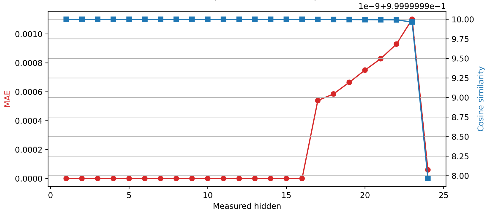
SmolLM2-1.7B-Instruct | Quantized layer 16 | float64 → int16
