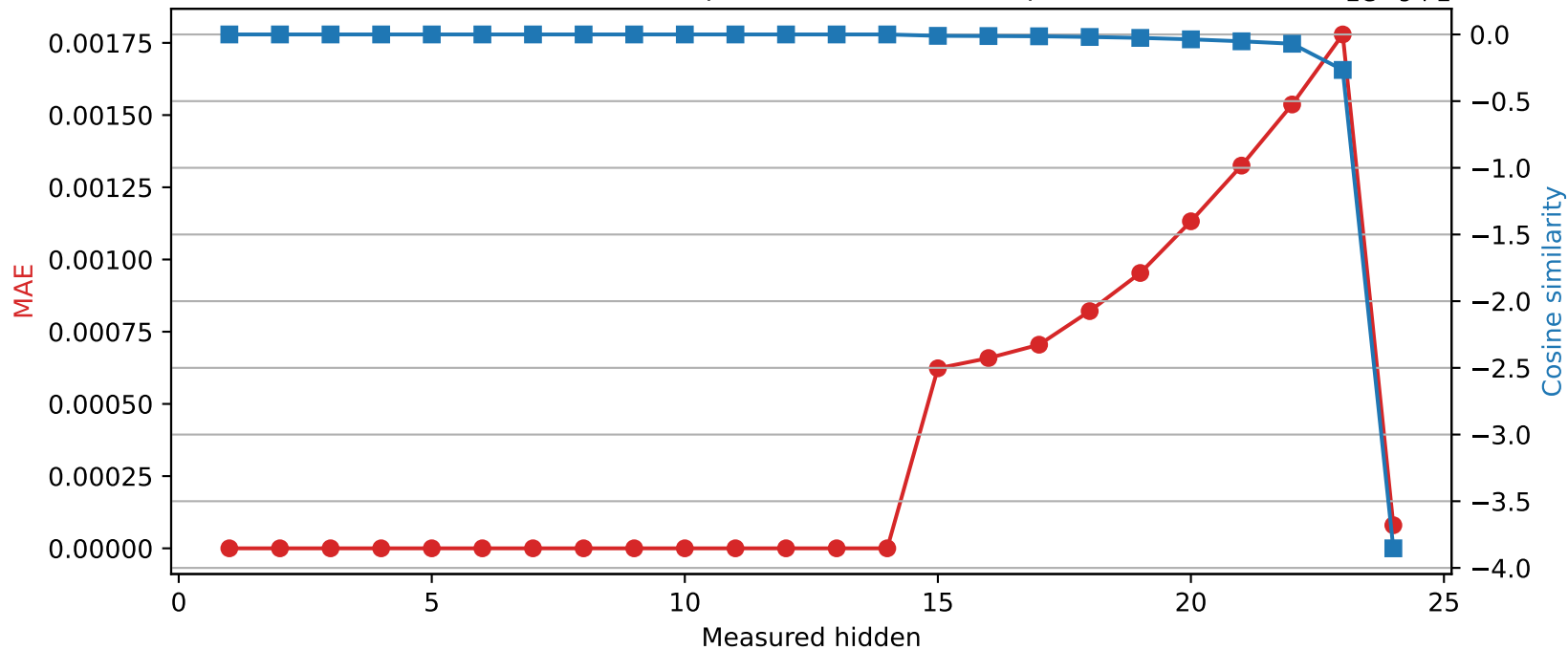
SmolLM2-1.7B-Instruct | Quantized layer 14 | float64 → int16
