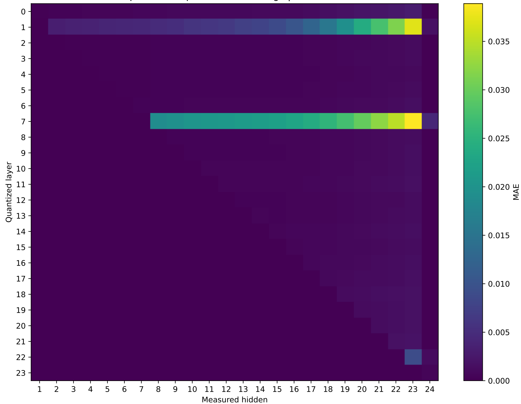
SmolLM2-1.7B-Instruct Prompt 3: MAE representation damage | float64 → int16
