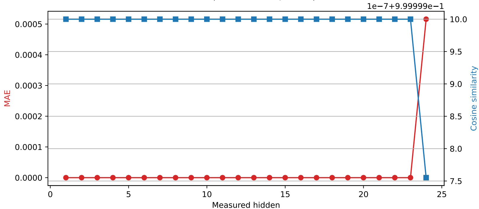
SmolLM2-1.7B-Instruct | Quantized layer 23 | float64 → int16
