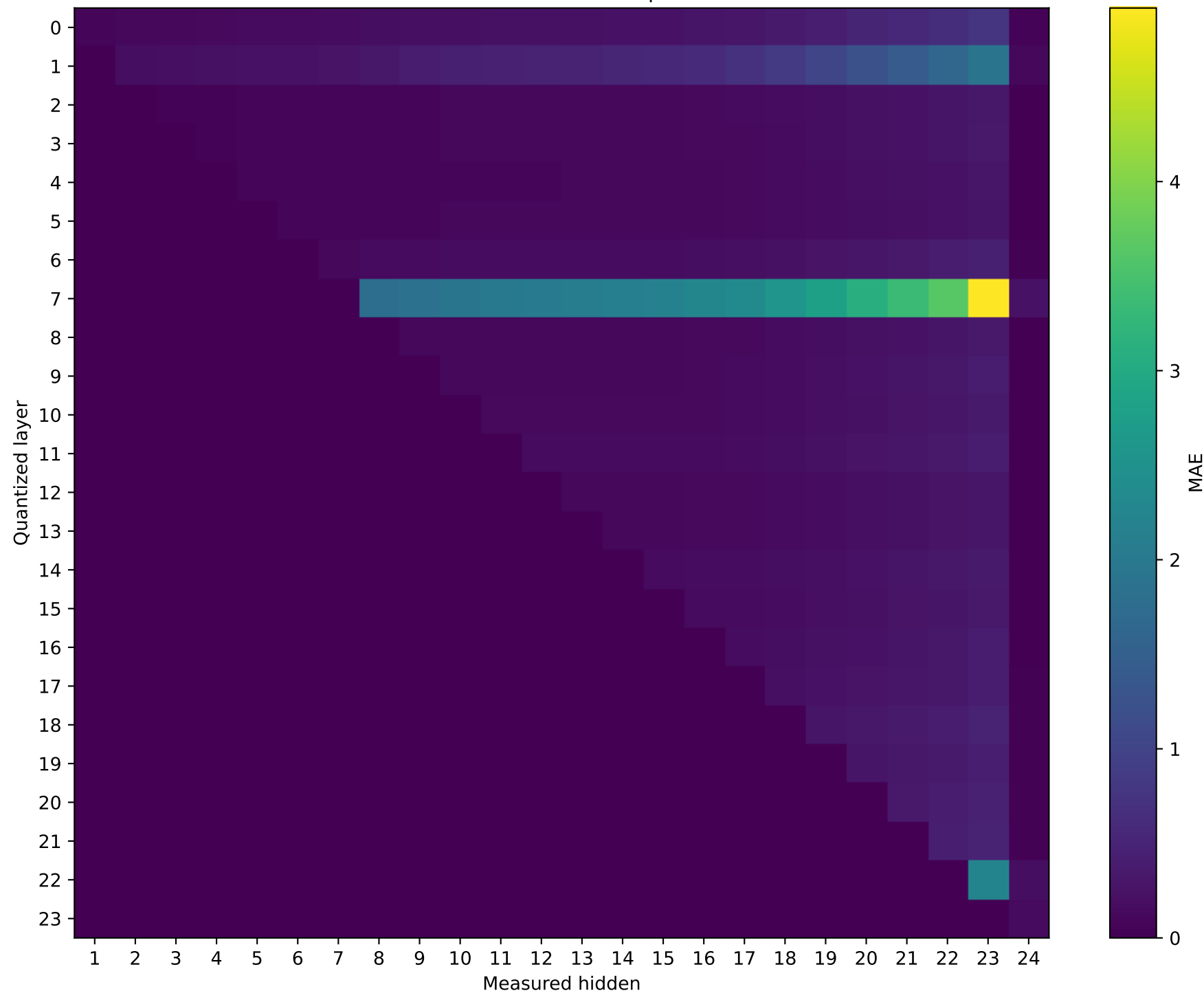
Model: SmolLM2-1.7B-Instruct | float16 \rightarrow int8
