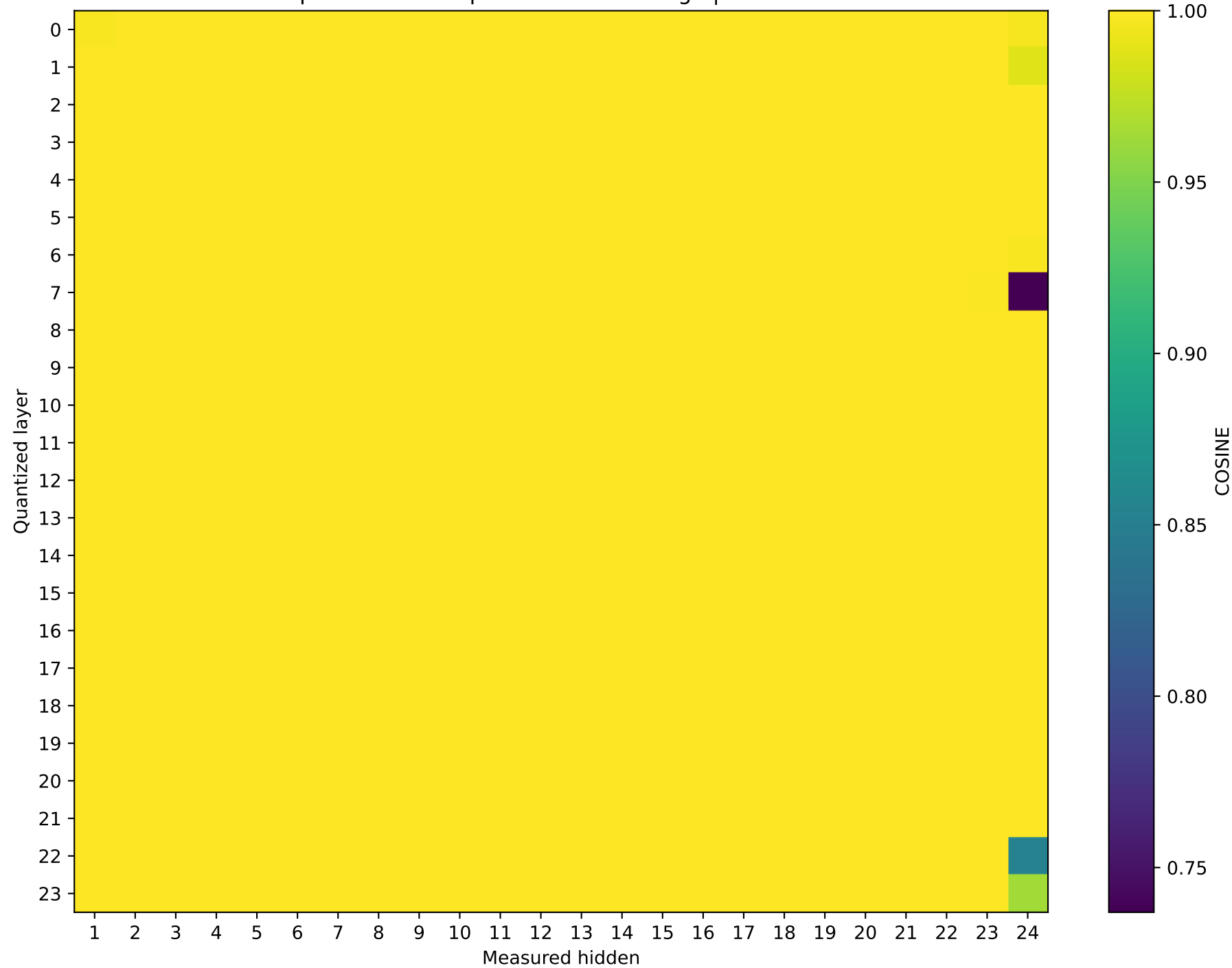
SmolLM2-1.7B-Instruct Prompt 0: cos sim representation damage | float16 → int8
