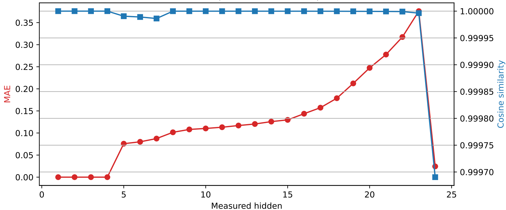
SmolLM2-1.7B-Instruct | Quantized layer 4 | float16 → int8
