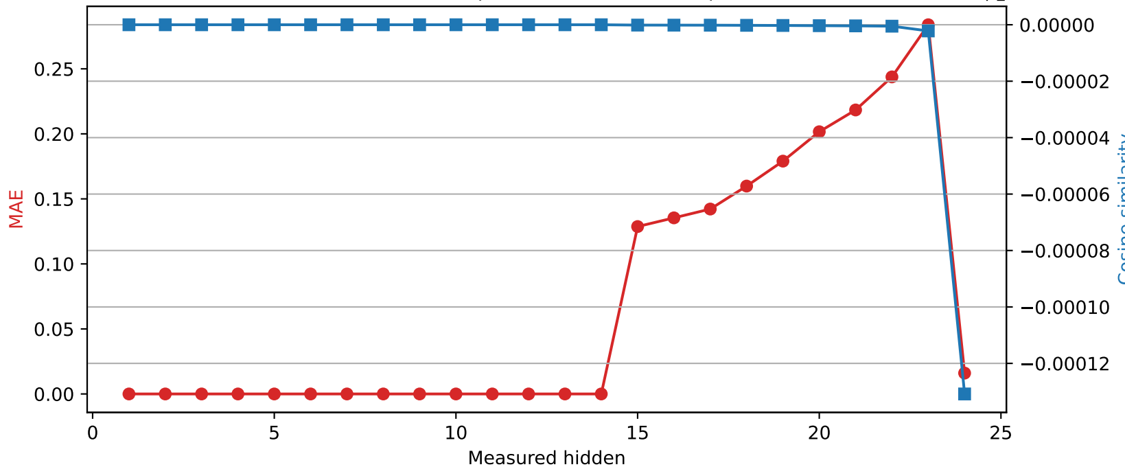
SmolLM2-1.7B-Instruct | Quantized layer 14 | float16 \rightarrow int8
