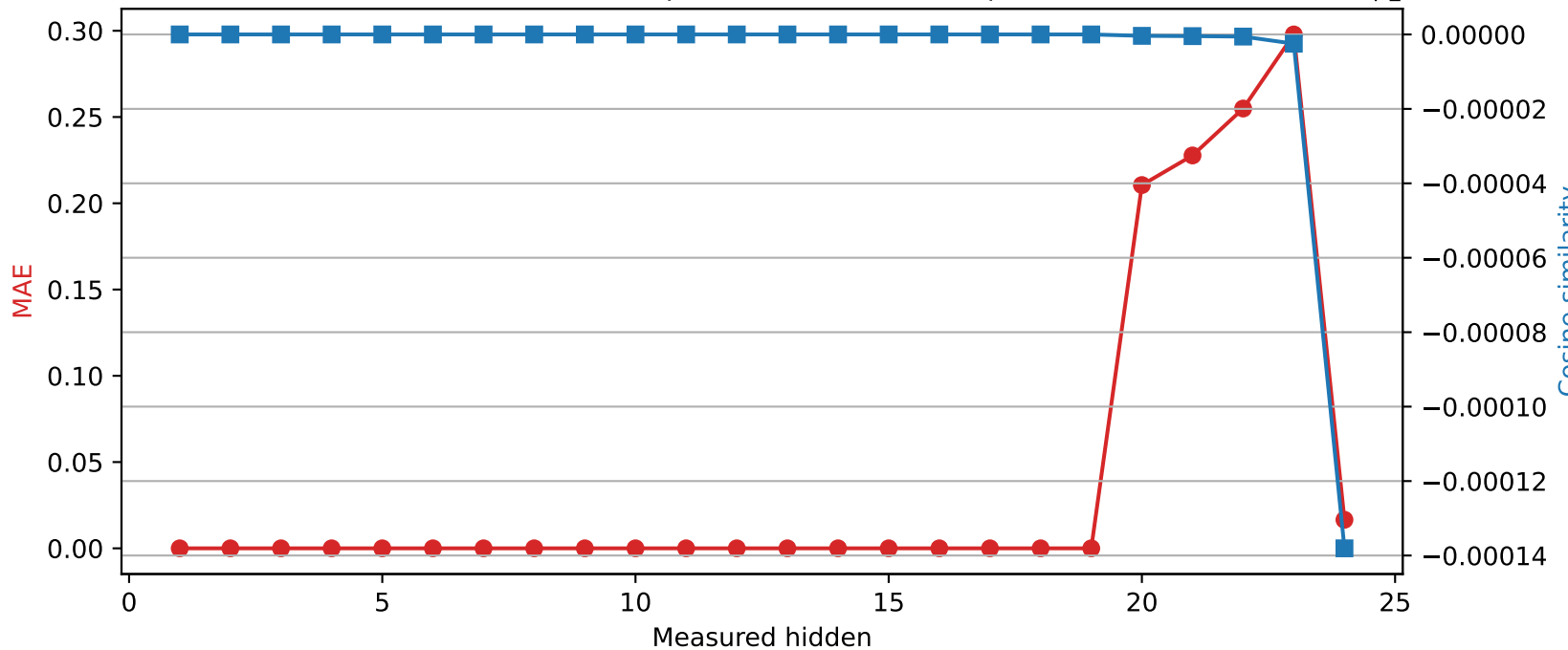
SmolLM2-1.7B-Instruct | Quantized layer 19 | float16 \rightarrow int8
