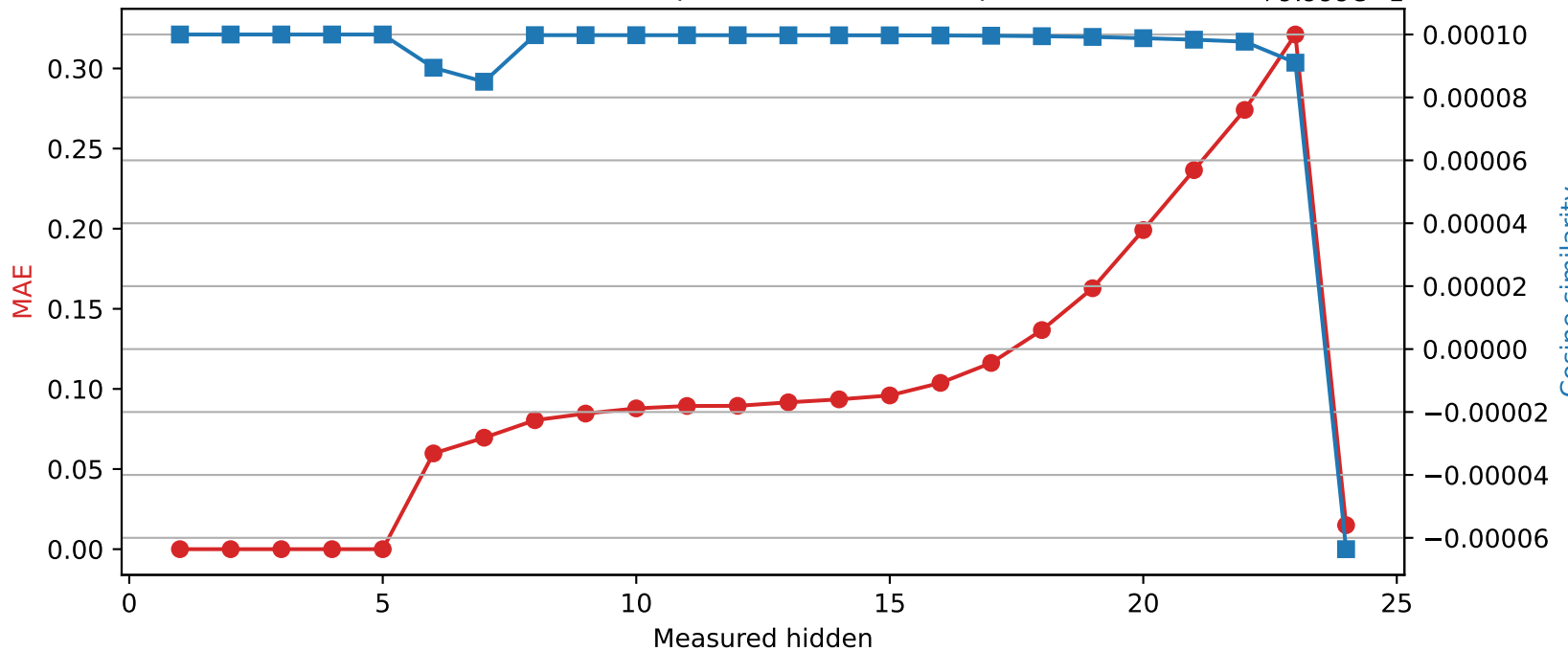
SmolLM2-1.7B-Instruct | Quantized layer 5 | float16 → int8
