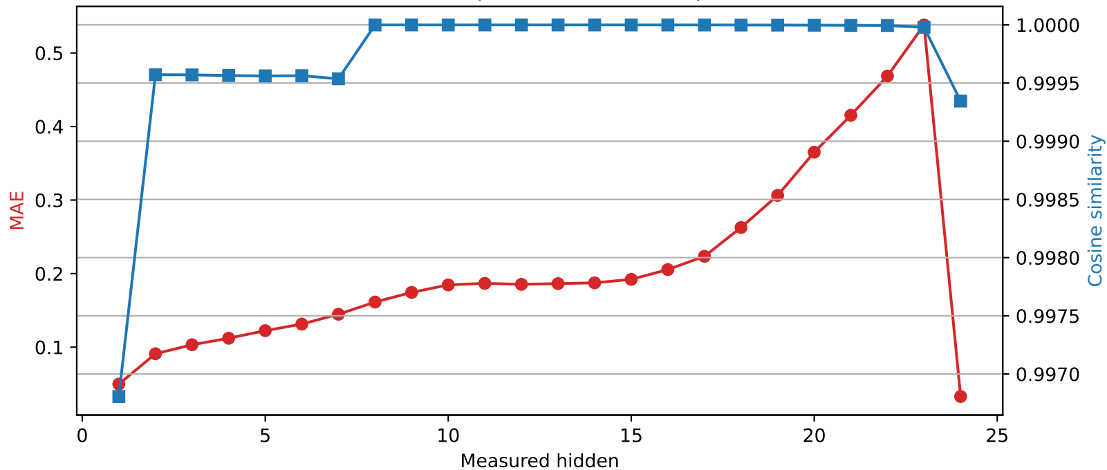
SmolLM2-1.7B-Instruct | Quantized layer 0 | float16 → int8
