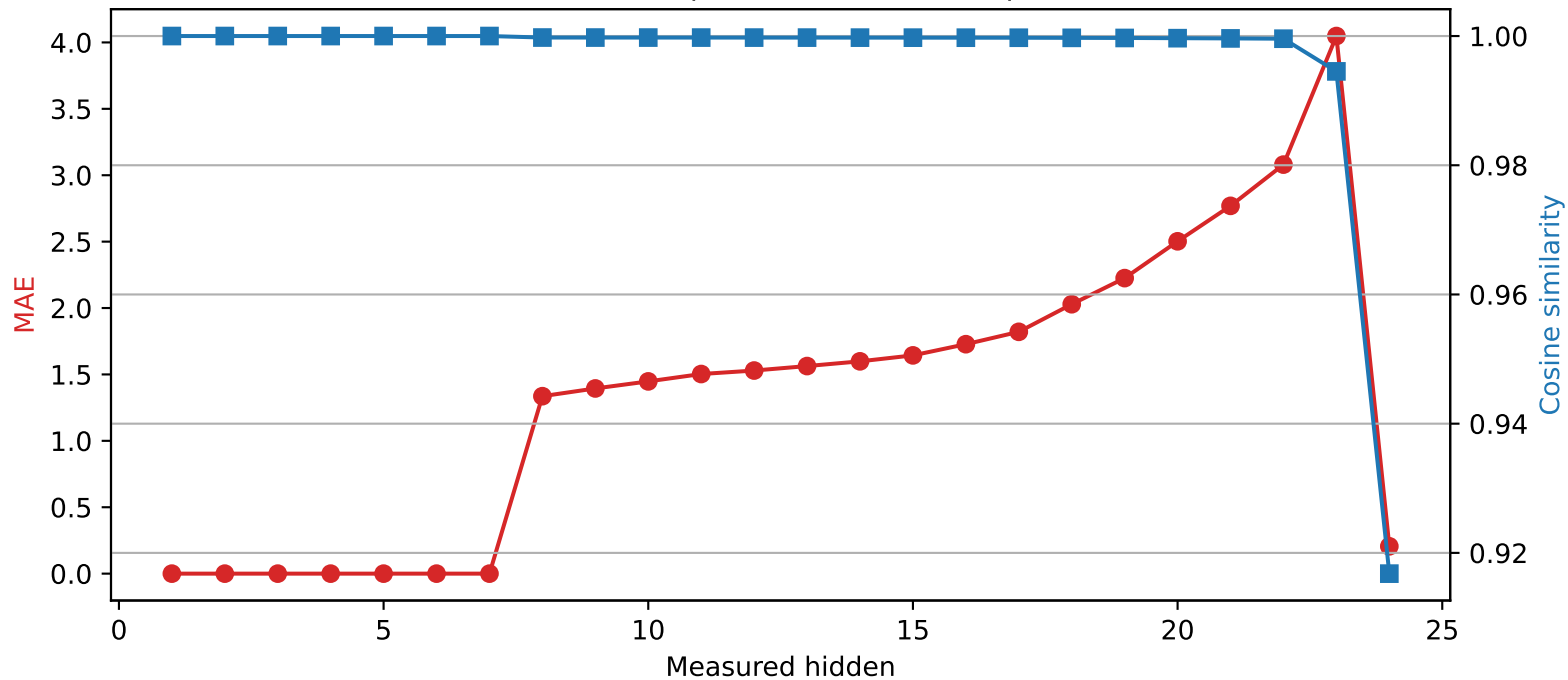
SmolLM2-1.7B-Instruct | Quantized layer 7 | float16 \rightarrow int8
