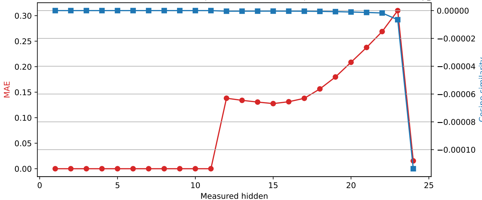
SmolLM2-1.7B-Instruct | Quantized layer 11 | float16 \rightarrow int8
