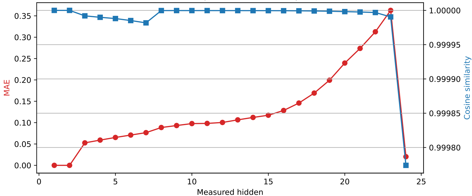
SmolLM2-1.7B-Instruct | Quantized layer 2 | float16 → int8
