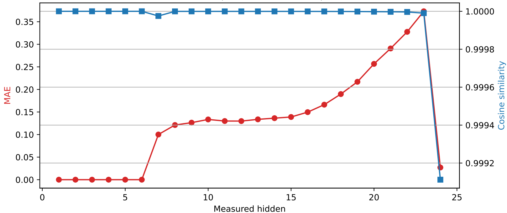
SmolLM2-1.7B-Instruct | Quantized layer 6 | float16 \rightarrow int8
