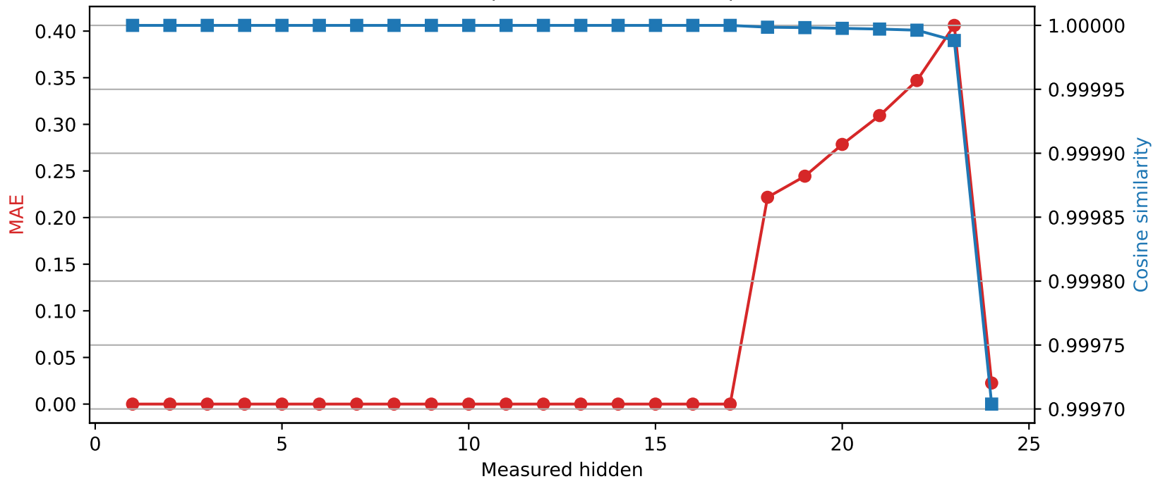
SmolLM2-1.7B-Instruct | Quantized layer 17 | float16 → int8
