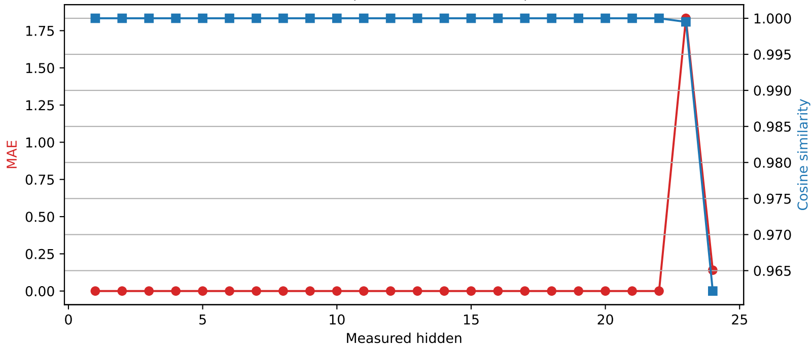
SmolLM2-1.7B-Instruct | Quantized layer 22 | float16 → int8
