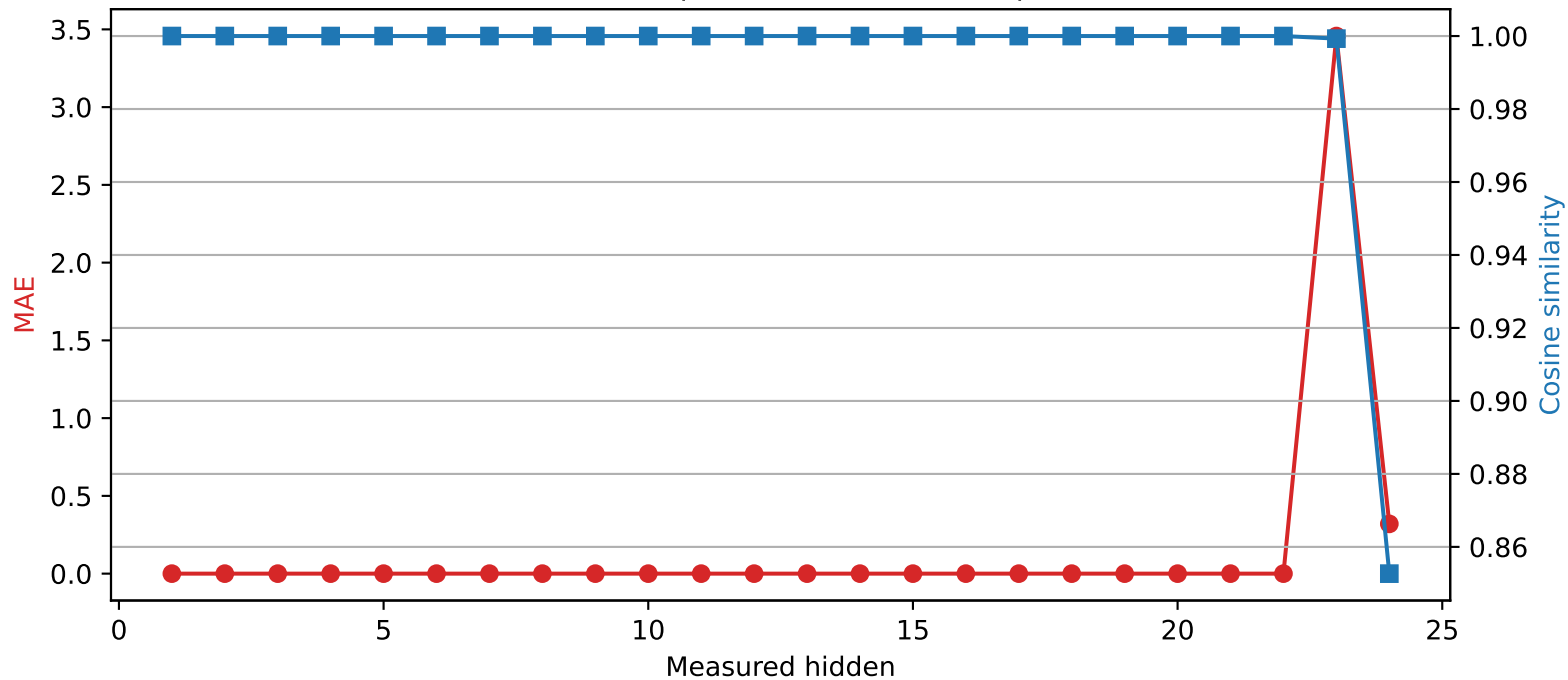
SmolLM2-1.7B-Instruct | Quantized layer 22 | float32 → int8
