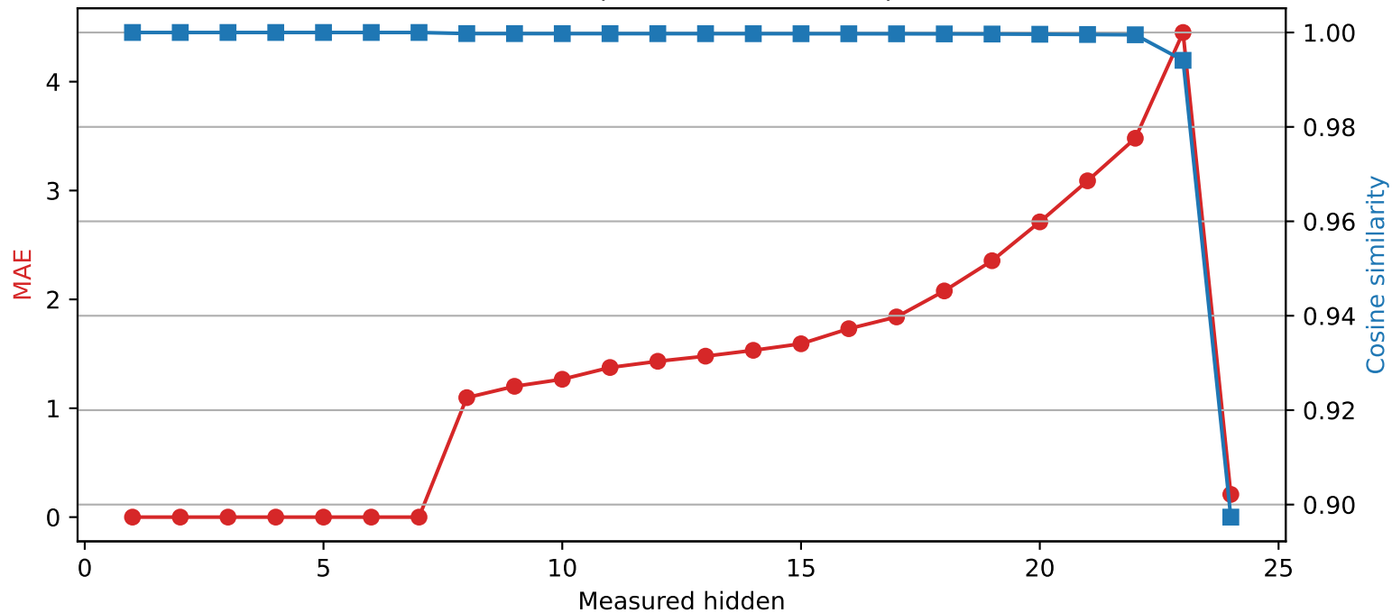
SmolLM2-1.7B-Instruct | Quantized layer 7 | float32 \rightarrow int8
