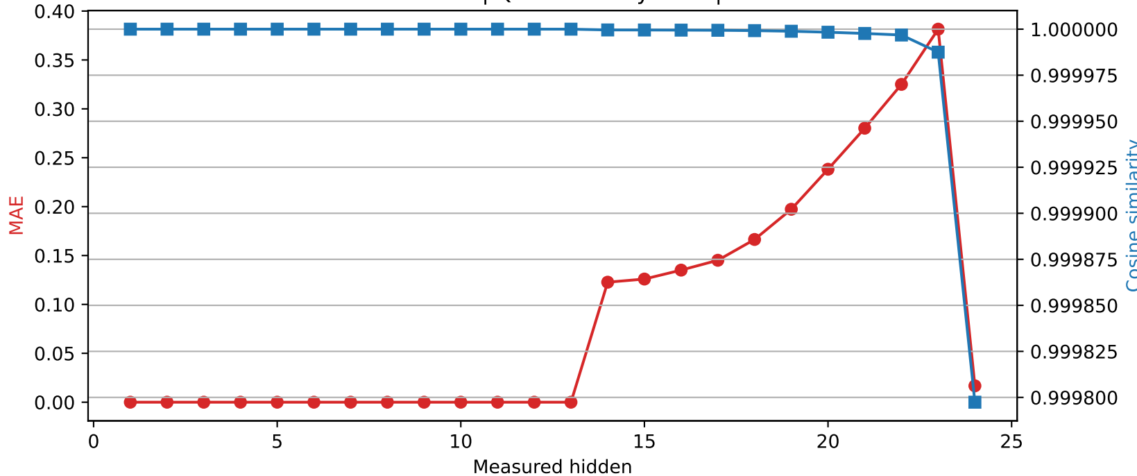
SmolLM2-1.7B-Instruct | Quantized layer 13 | float32 → int8
